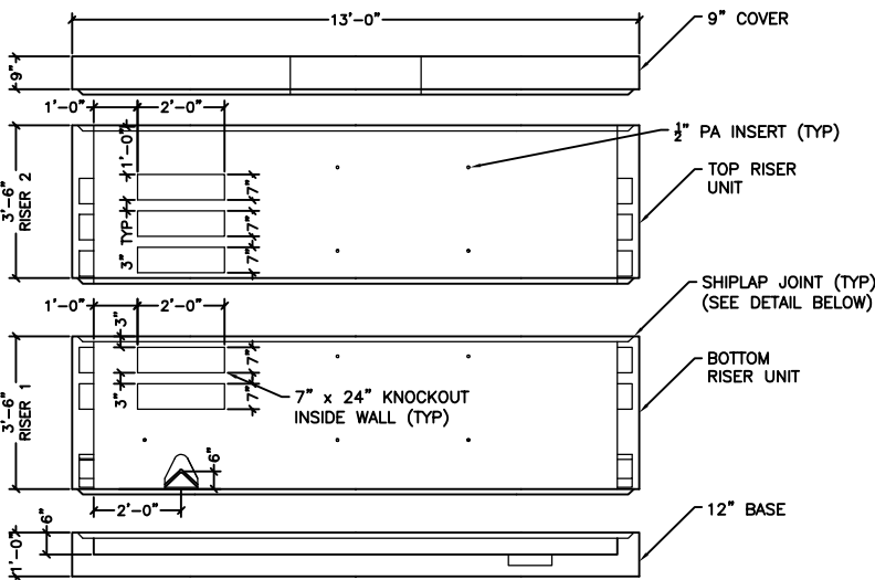
ELEVATION VIEW (SECTION A-A)
