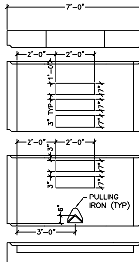
SIDE ELEVATION VIEW (SECTION B-B)
