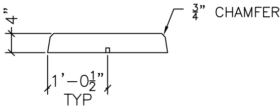
ELEVATION VIEW (SECTION A-A)
