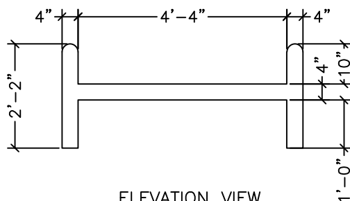
ELEVATION VIEW
