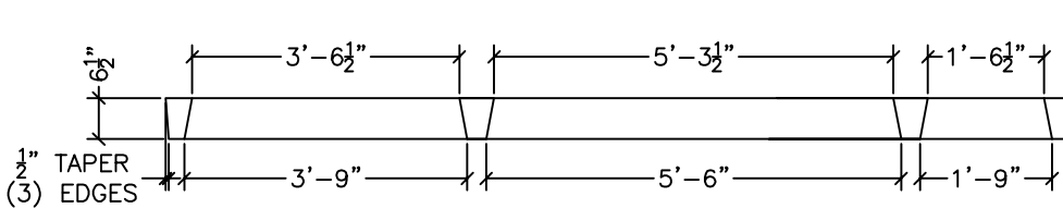
ELEVATION VIEW (SECTION A-A)
