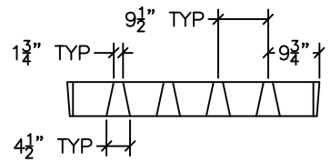
SIDE ELEVATION VIEW (SECTION B-B)
