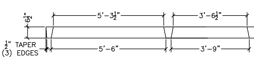
ELEVATION VIEW (SECTION A-A)
