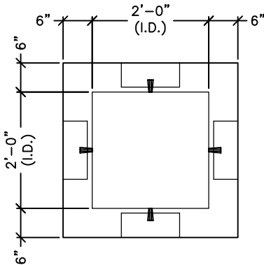
PLAN VIEW (COVER REMOVED)
