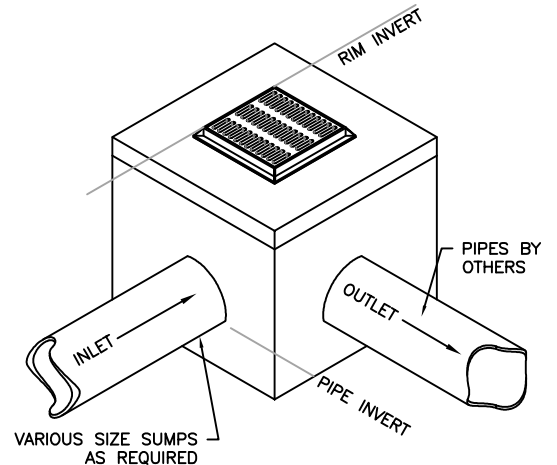
IN-FIELD VIEW
