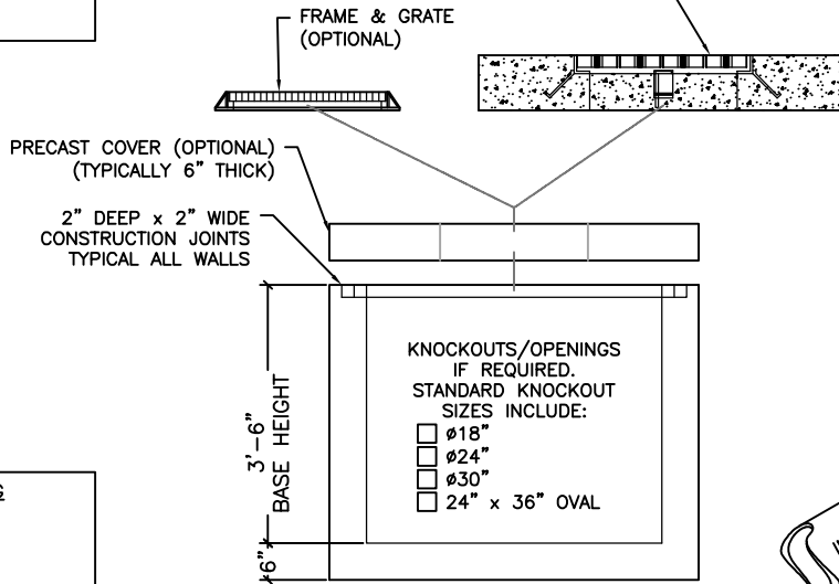
ELEVATION VIEW
