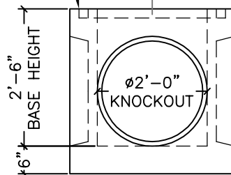
ELEVATION VIEW
