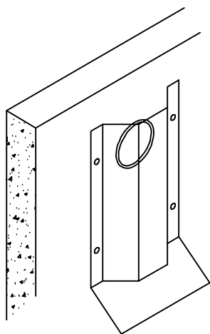
Isometric View Of Plastic Baffle Attached To Inside Of Septic Tank
