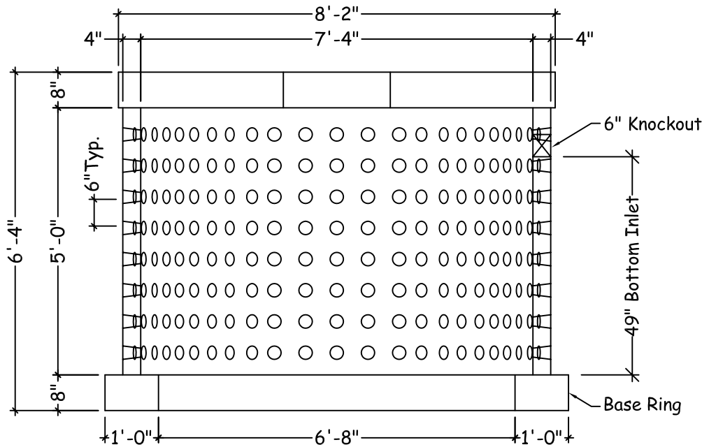
Elevation View
