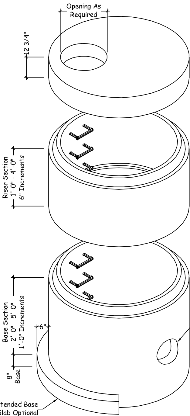
Isometric View
