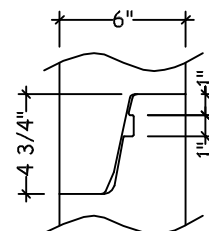
Joint Detail
