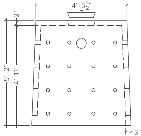
SECTION VIEW 'B'
